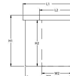
TA1233 Rectangular Tank
